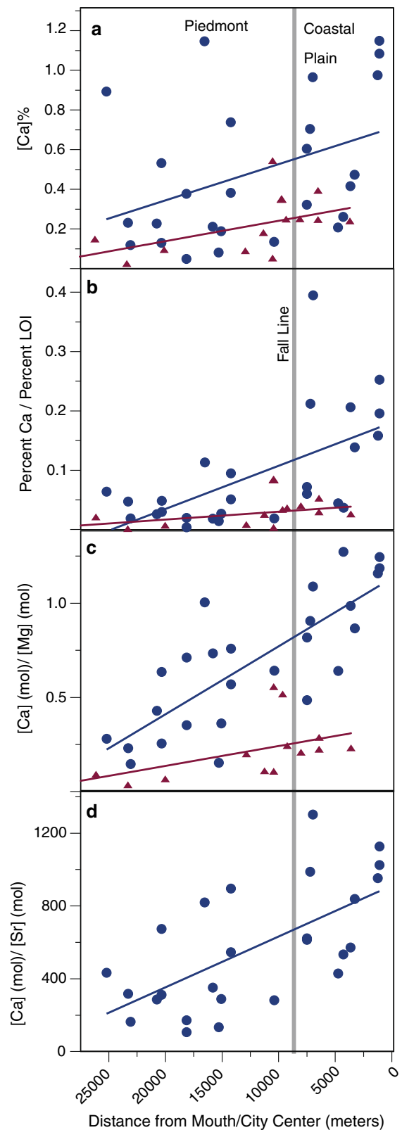
Fig. 3 Plots showing the concentration of Ca along the riparian and forested patch transects through the Gwynns Falls/Baltimore City and County. Results from this study are shown as circles . Triangles represent data from a transect of soils under forested patches, with distance calculated from the city center as reported here (Pouyat et al. 2008). a shows raw Ca concentrations, and the other panels show Ca normalized with material lost on ignition ( b ), magnesium ( c ), and strontium ( d ). Strontium concentrations were not measured in the upland forest plot transect. Linear fits of the data series as a function of distance are as follows: Ca a This study ( r^2 = 0.15 , p < 0.05 ), forested patches ( r^2 = 0.32 , p < 0.05 ). Ca/LOI b This study ( r^2 = 0.35 , p < 0.005 ), forested patches ( r^2 = 0.21 , p < 0.05 ). Ca/Mg. c This study ( r^2 = 0.63 , p < 0.0001 ), forested patches ( r^2 = 0.29 , p < 0.05 ). Ca/Sr d This study ( r^2 = 0.41 , p < 0.0005 )
