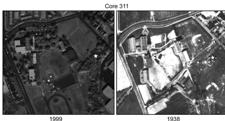
Fig. 5 Aerial photos showing local land uses around transect 311. Note that while contemporary imagery shows a forested riparian zone, this core was taken from an area that was athletic fields as late as 1938, which can explain some of the observed chemistry
