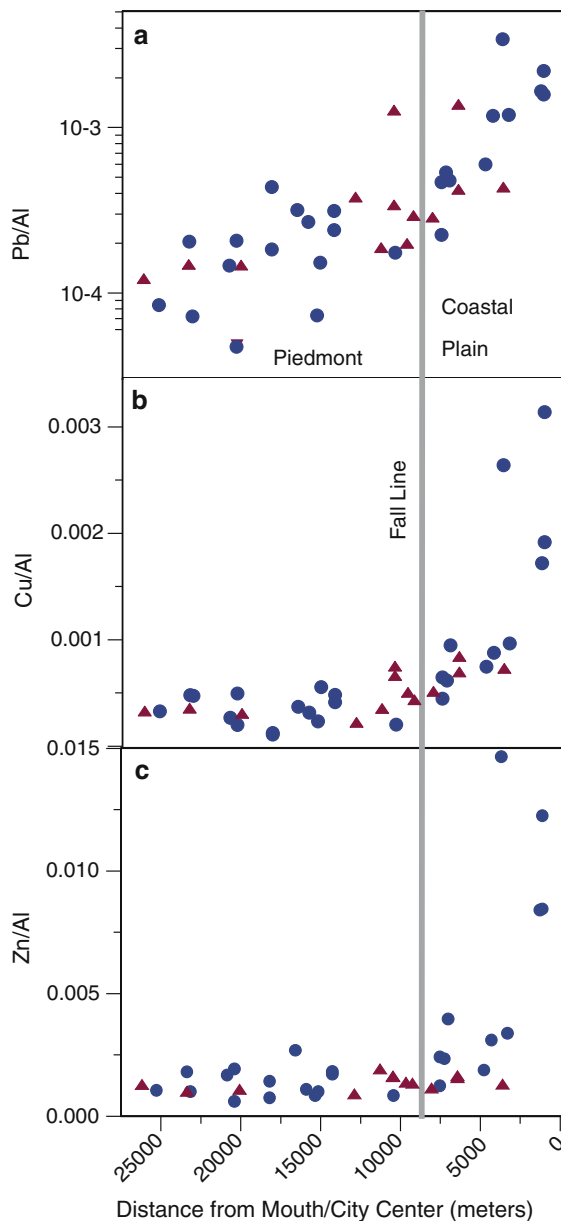
Fig. 4 Concentrations of urban suite trace metals along Gwynns Falls transect. a–c Shows lead, copper, and zinc (respectively) concentrations normalized with aluminum concentration (a proxy for clay concentration and therefore surface area). Results from this study are shown as circles . Triangles represent data from a transect of soils under forested patches, with distance calculated from the city center as reported here (Pouyat et al. 2008)
